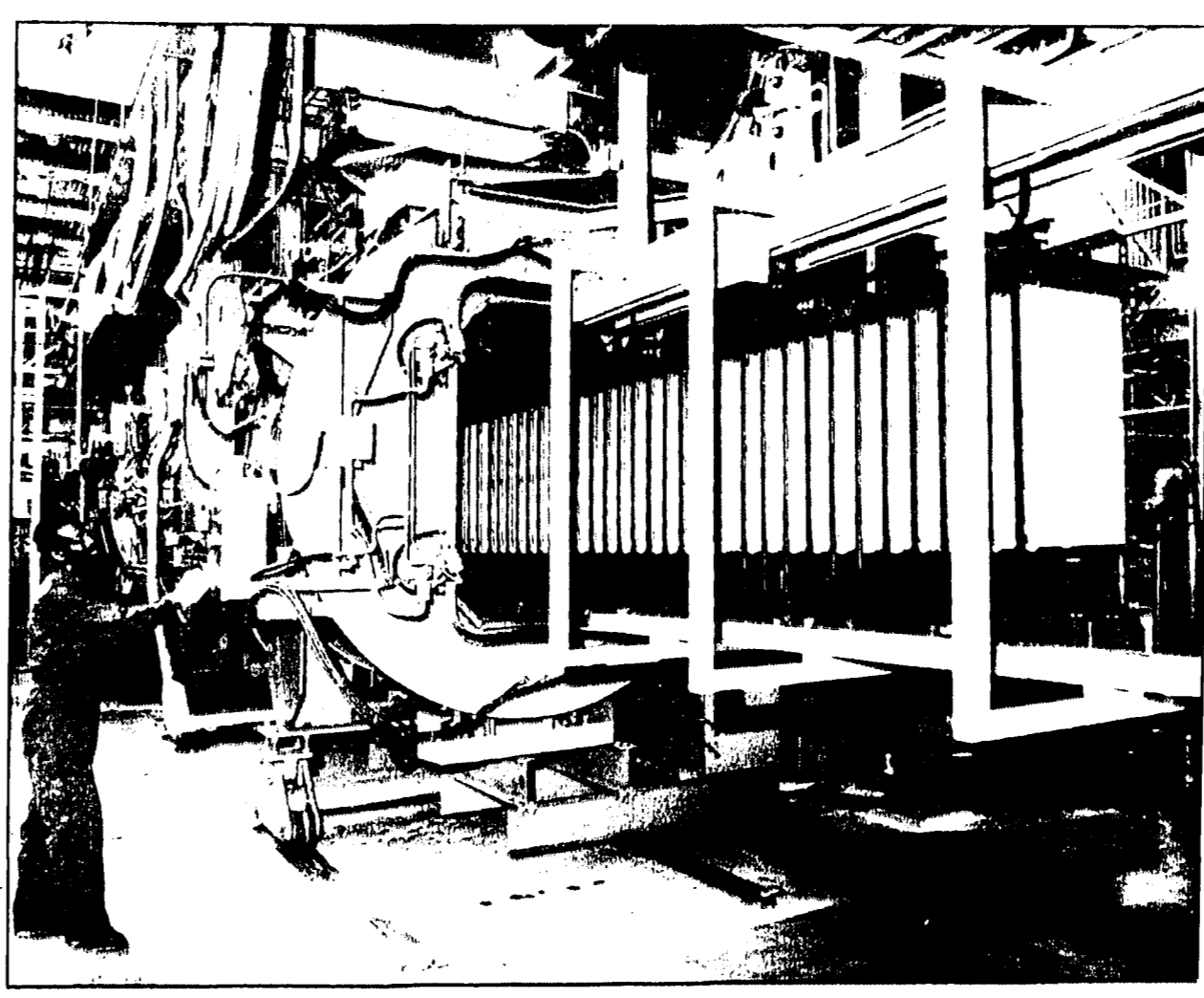
Aluminum radiator cores enter preheat chamber of vacuum brazing furnace at Ford's Sheldon plant
