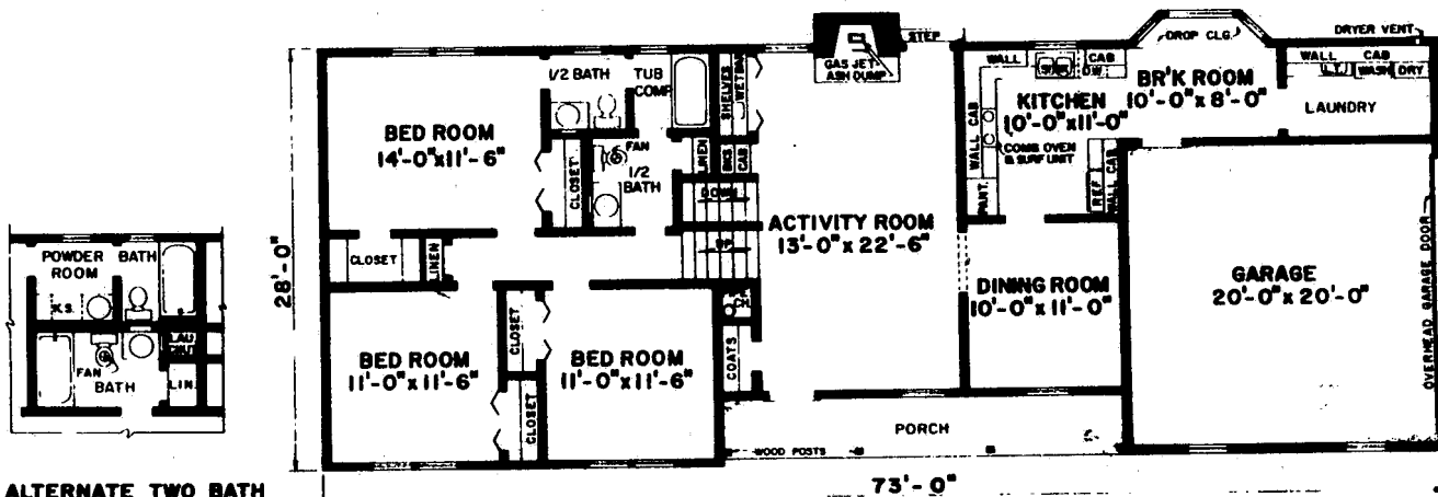
ALTERNATE TWO BATH
