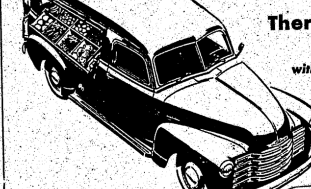
LIGHT-DUTY CANOPY EXPRESS Model 3107—116-inch wheelbase, Maximum G.V.W. 4600 lbs. Also available in Medium-Duty Model 3807—137-inch wheelbase, Maximum G.V.W. 6700 lb.
