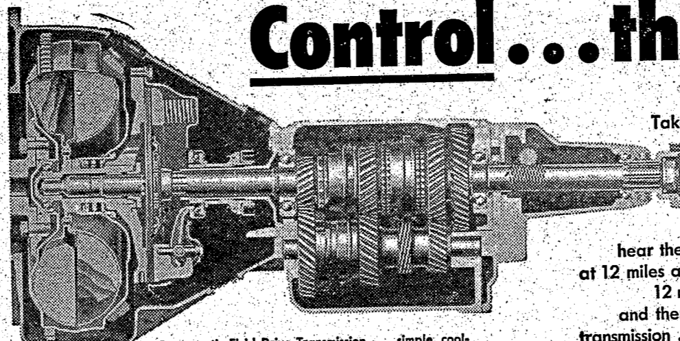
Prestomatic Fluid Drive Transmission... simple, cool-running, with three rugged compact units designed with a minimum of moving parts... a great Fluid Drive, the Safety Clutch, and Prestomatic Transmission. Ruggedly built for trouble-free service.
