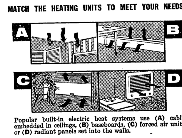
POPULAR built-in electric heat systems use (A) cable embedded in ceilings, (B) baseboards, (C) forced air units or (D) radiant panels set into the walls.
