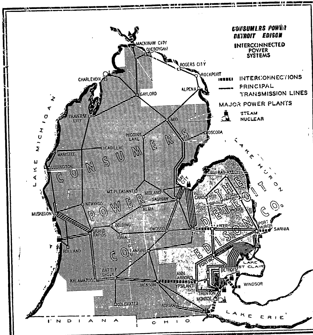
This map shows the total interconnected electric pool area served by Detroit Edison and Consumers Power. The new joint operational agreement between the two companies will further coordinate and reinforce the existing electric transmission network throughout the entire Lower Peninsula of Michigan.
