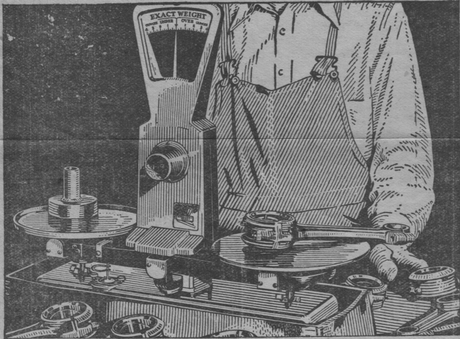
Chevrolet connecting rods are matched in sets of six to within one-quarter ounce, and are individually fitted by hand to the crankshaft. Bearings are of Babbitt metal cast into the rods under heavy air pressure and at 800° Fahrenheit.
