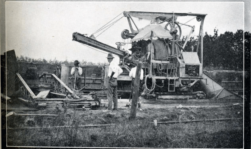
Concrete paving equipment, John R Road
