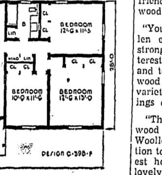
A SMALL HOUSE PLANNING BUREAU DESIGN NO. C-398-F
