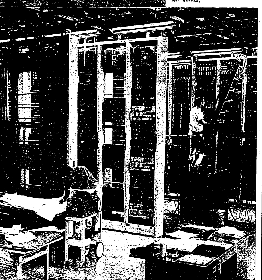
Hundreds of man hours of work were required to install and test equipment in Northville's new exchange building before the switch from manual to dial service. One company technician pictured here checks wiring blueprints and relays circuit information to a fellow worker.
