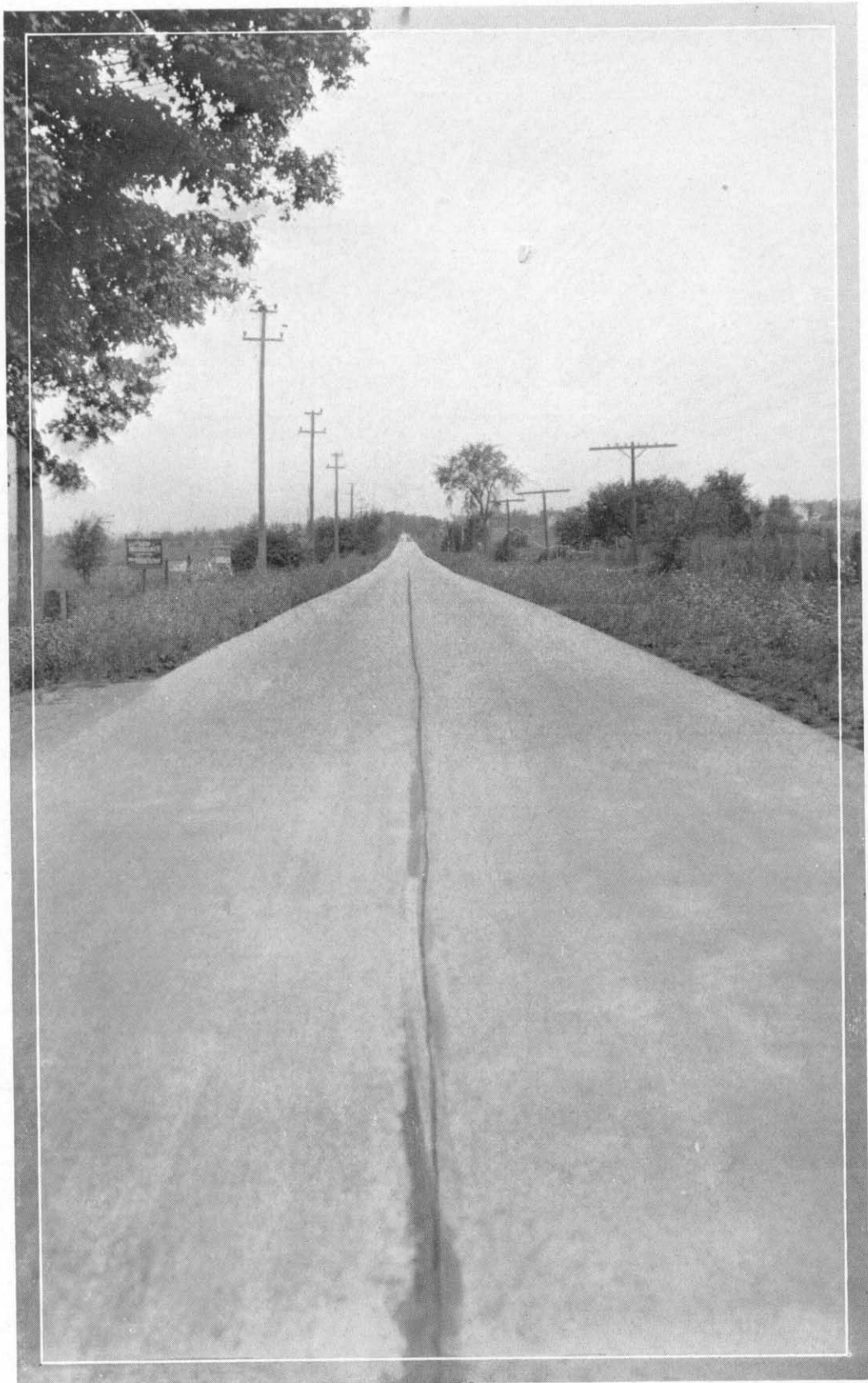
SOUTHFIELD ROAD SHOWING CENTER CONTRACTION JOINT
