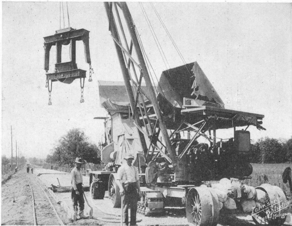
Forty-four cubic ft. mixer used on Auburn road, concrete.
