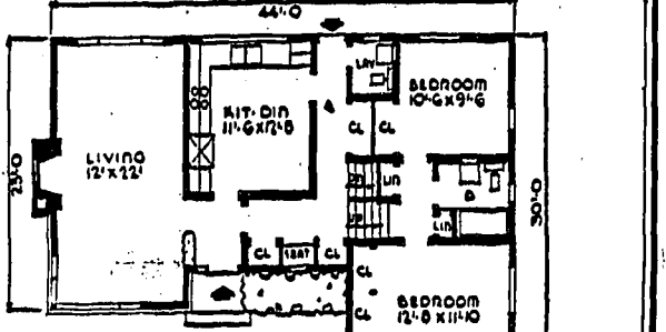
DESIGN C-495-S. Designed for a level lot, this split-level house provides four bedrooms. Two on the first floor have wardrobe type closets and a full bath. A lavatory and large coat closet are located at the rear entry. The kitchen features built-in oven, counter top cooking unit, generous cabinets and space for dining. Floor area is 1079 square feet, culage is 20 1/2" x 10 1/2" feet.
